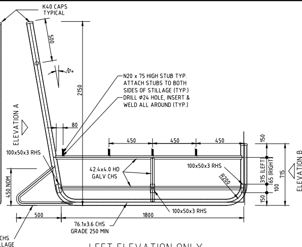
LEFT ELEVATION ONLY 1:20
