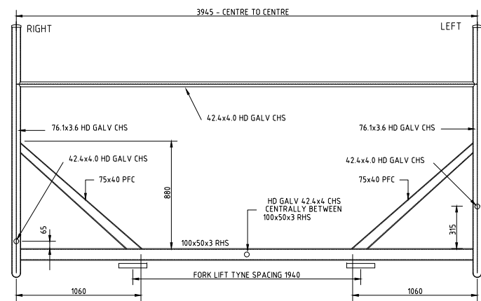
ELEVATION A 1:20
