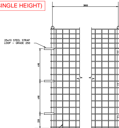
PANEL DETAIL 1:10
