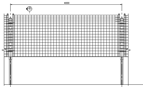
DEBRIS FENCE ASSEMBLY 1:20
