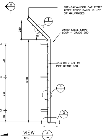
PANEL DETAIL 1:10
